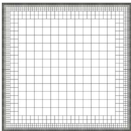
Fig. 2 Initial computational grid of the square cavity
