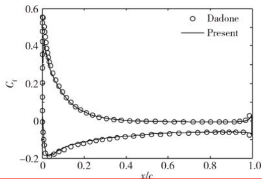
Fig. 11 Skin friction coefficient distributions on the surface of the NACA0012 airfoil for case 1
